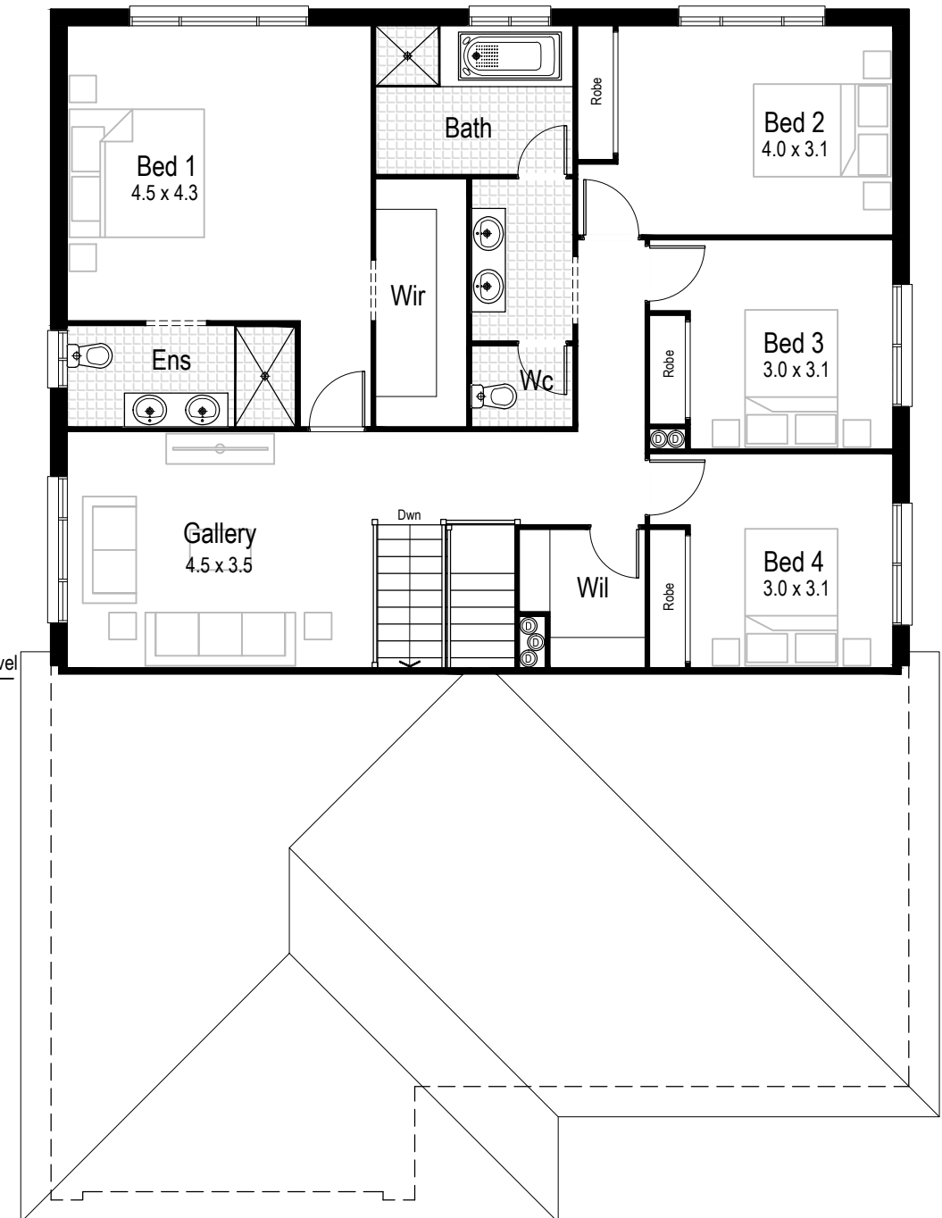
First Floor
